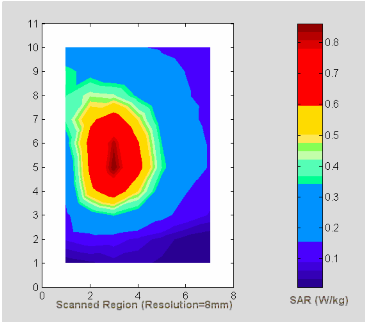
Fig. 11c. Repeated measurements for the three coarse scans each lasting 20 minutes at 5.32 GHz for the Proxim Model 8460 Cardbus Card inserted in a laptop computer pressed against the flat body phantom. Measurement 3 (see Table 2c for the peak 1-g SAR).
