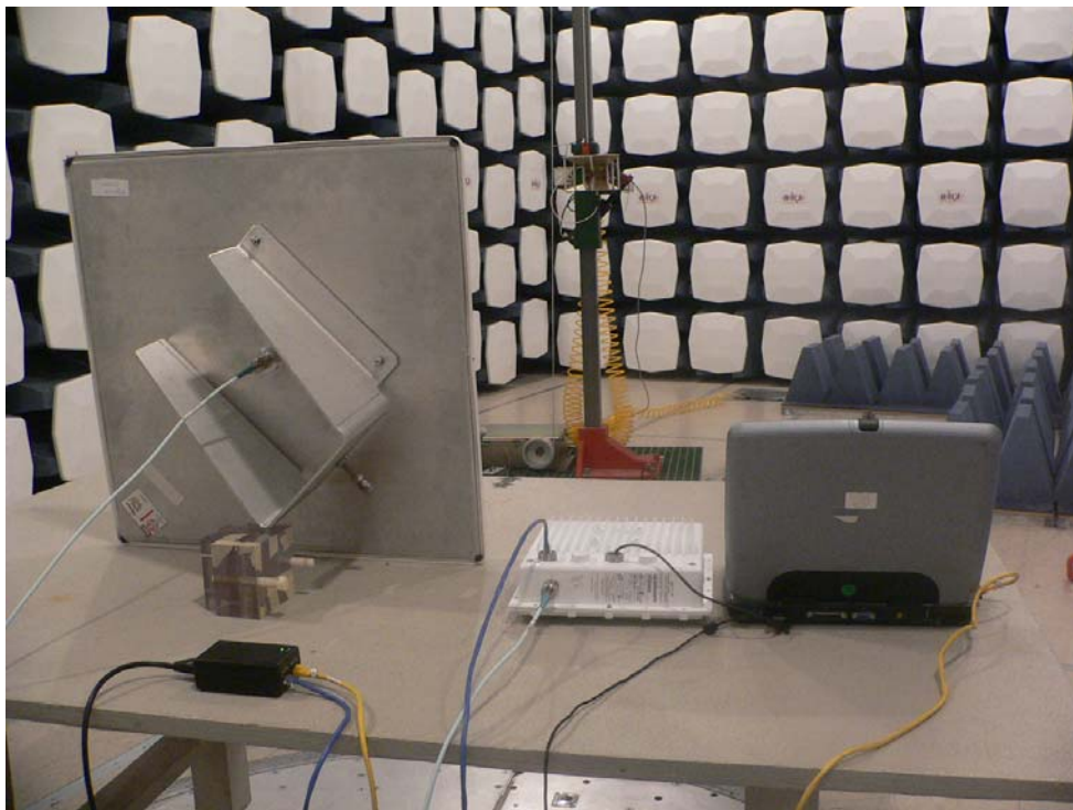
Radiated Emission – Rear View (Panel Antenna 28.5 dBi )
