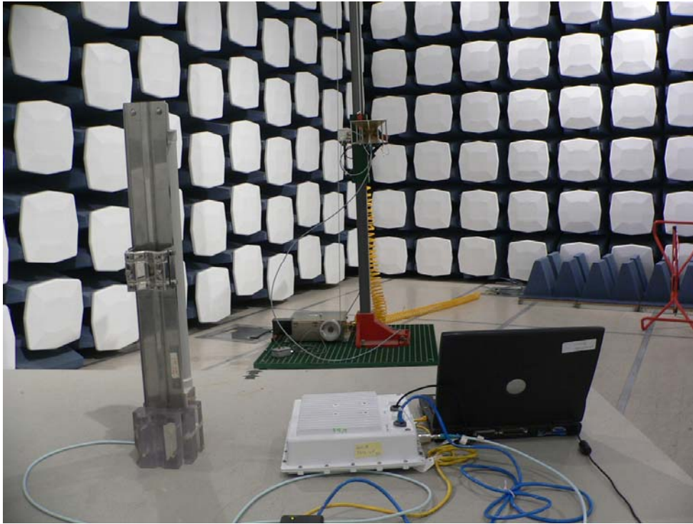
Radiated Emission – Rear View (Sector Antenna 17.0 dBi )
