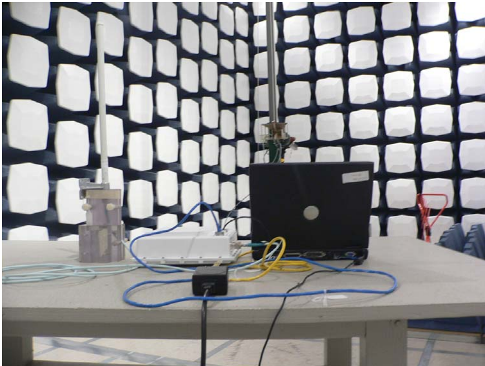
Radiated Emission – Rear View (Omni Antenna 10.0 dBi )
