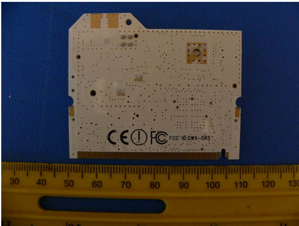
RF Board With Shield Off – Back
