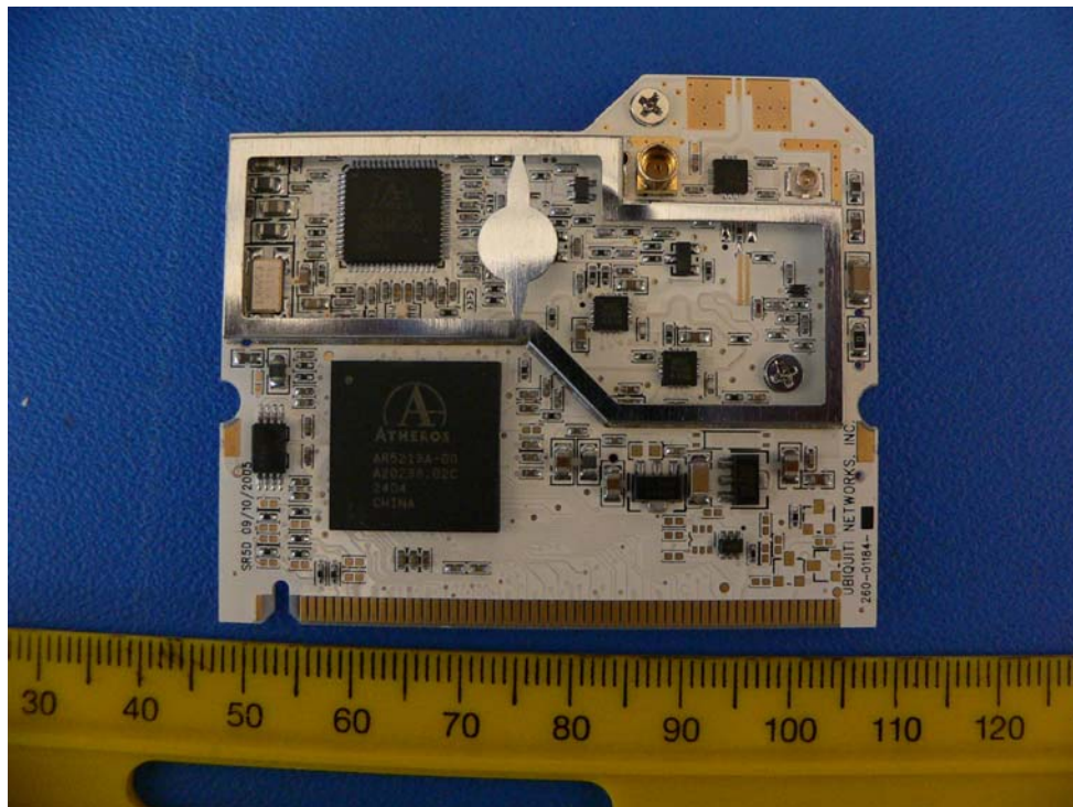
RF Board with Shield Off – Front
