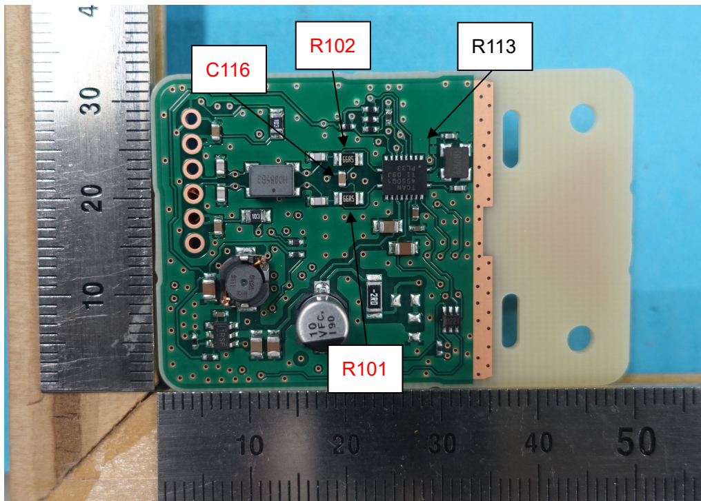
Top : R113 Not mounted(Pattern short)
