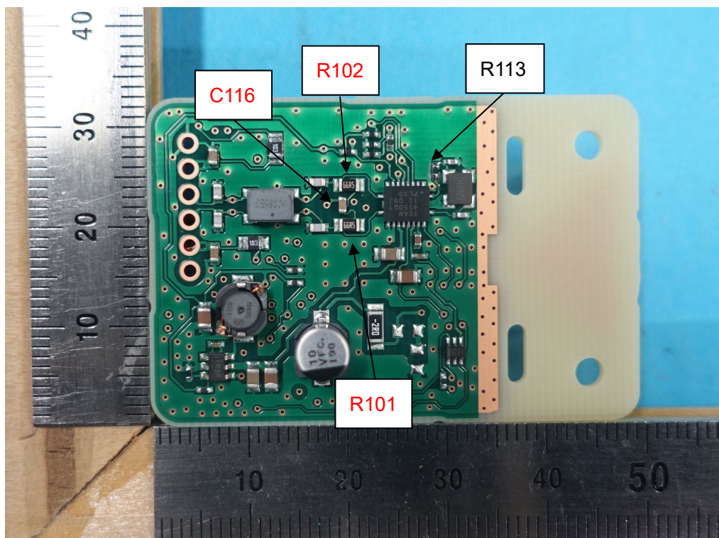
Top : R113 Mounted(Pattern open)
