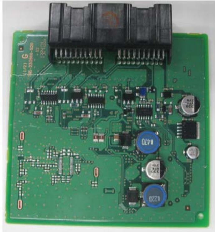
Component Side
