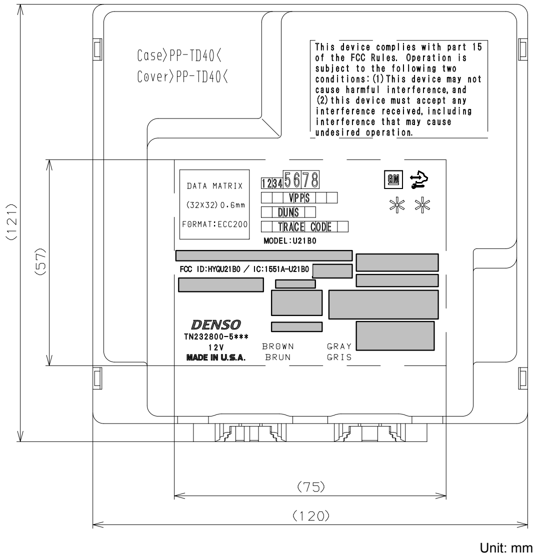
Fig. Marking location and layout of UPE
