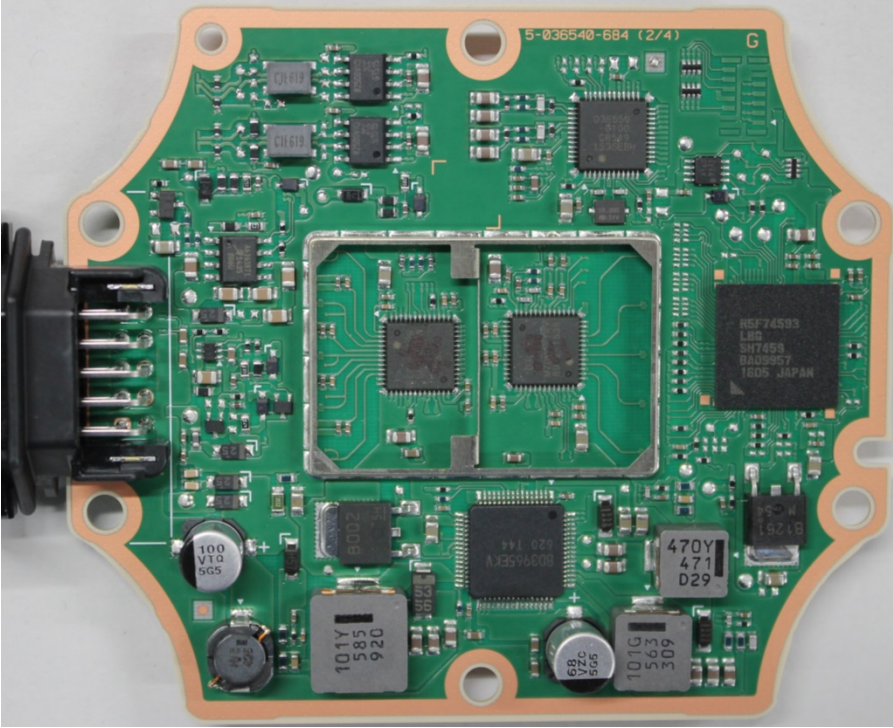
Component side
