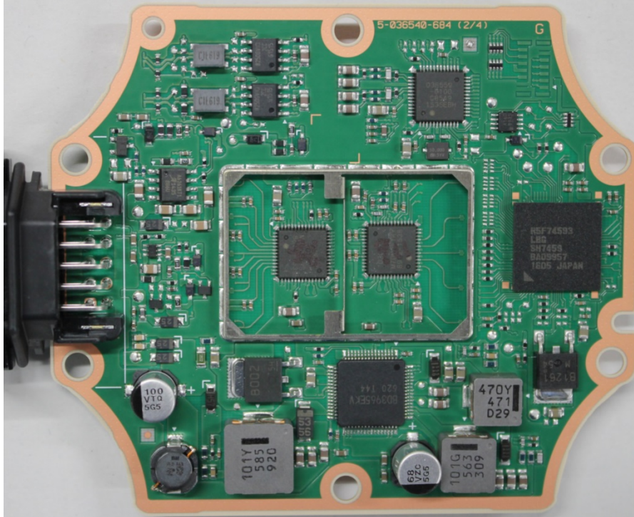
Component side
