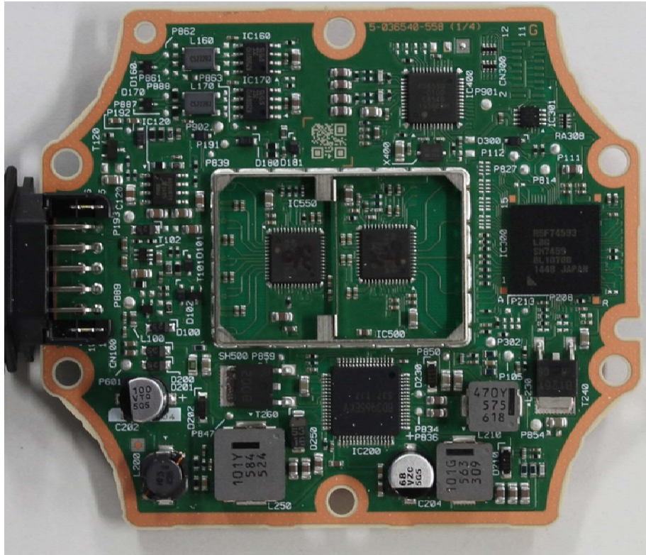
Component side
