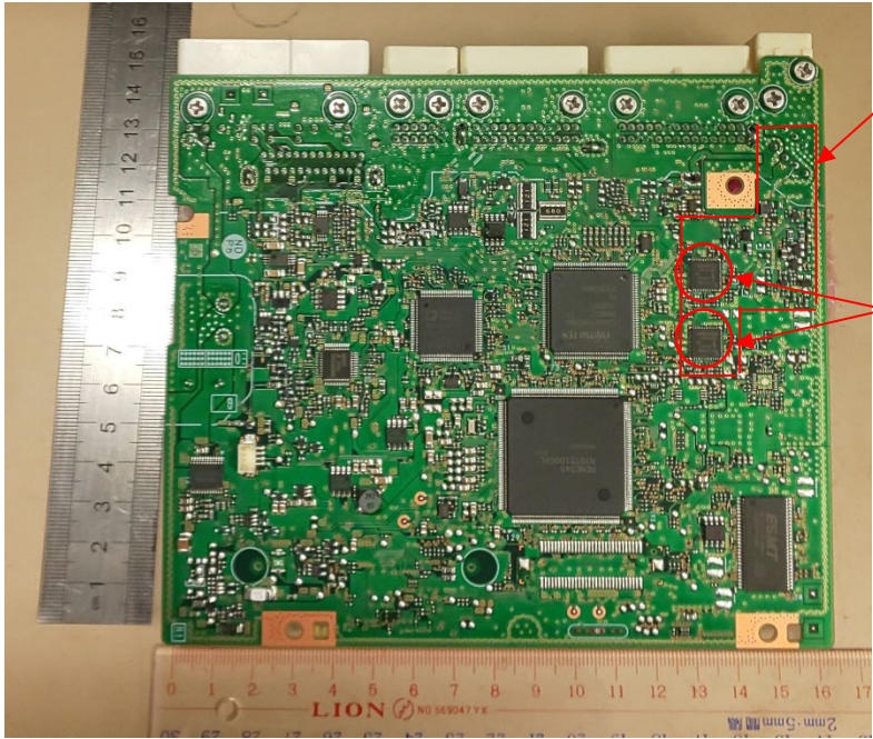
Solder Side
