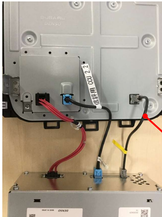
Connection part of the CCU and CID
