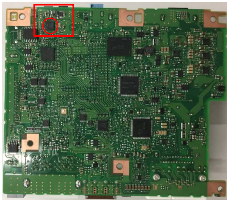
Solder Side
