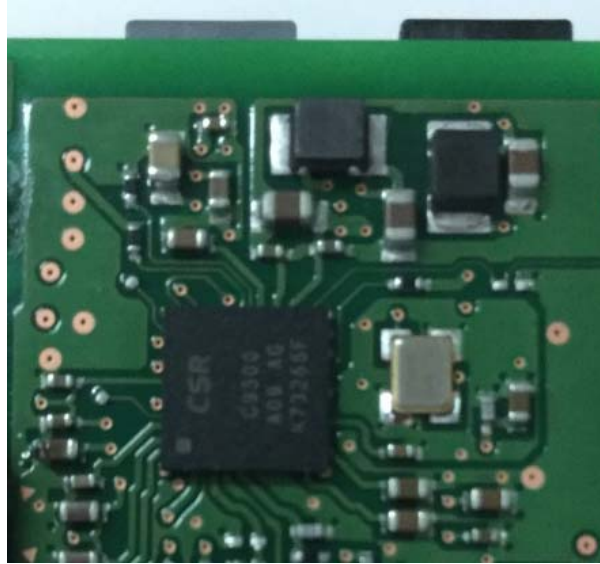
Bluetooth and WiFi Module IC
