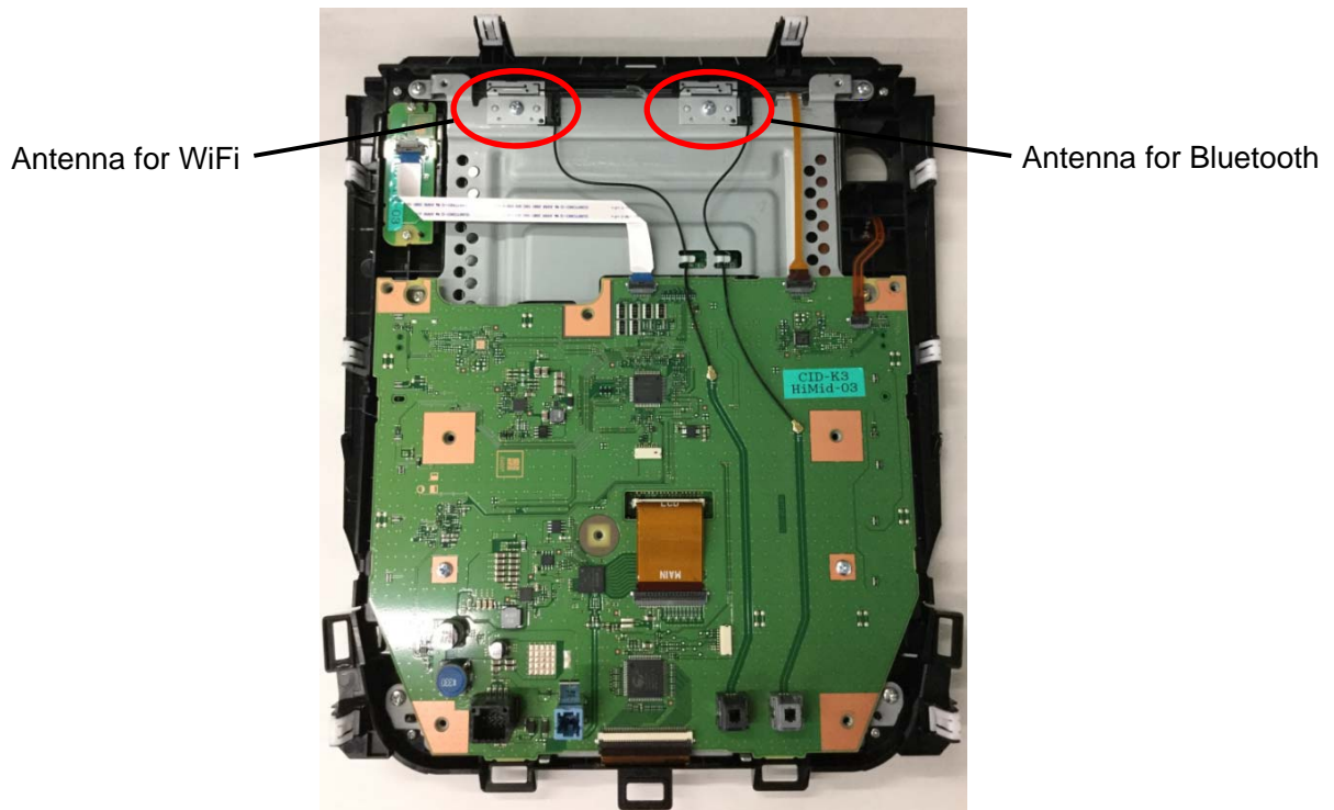
CID(Center Information Display) internal
