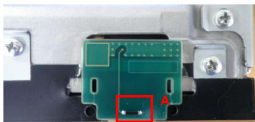
Bluetooth antenna
