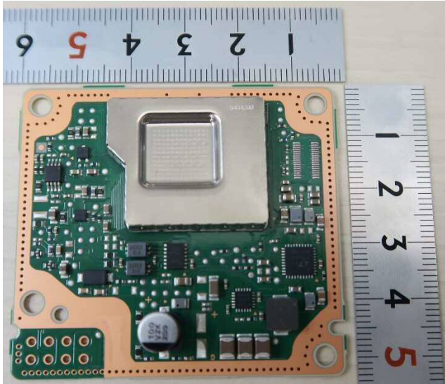
Component side (With Shield)
