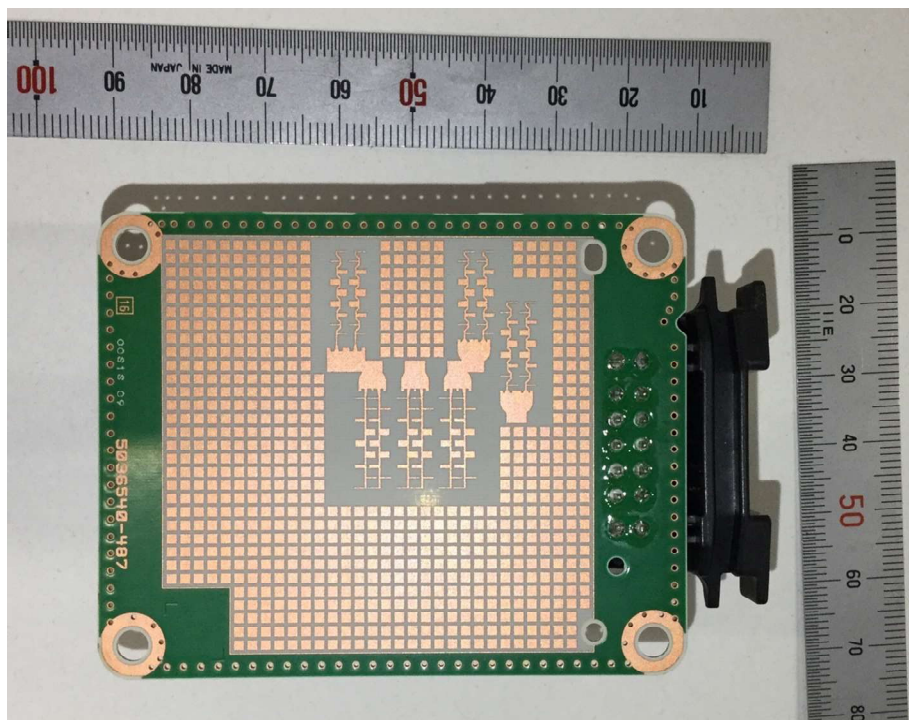
Antenna side
