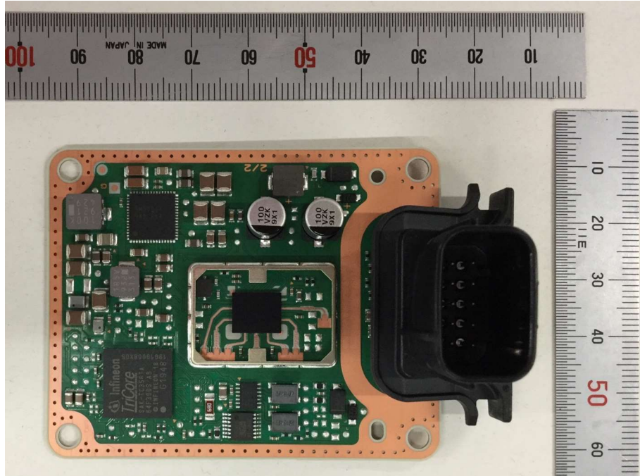
Component side
