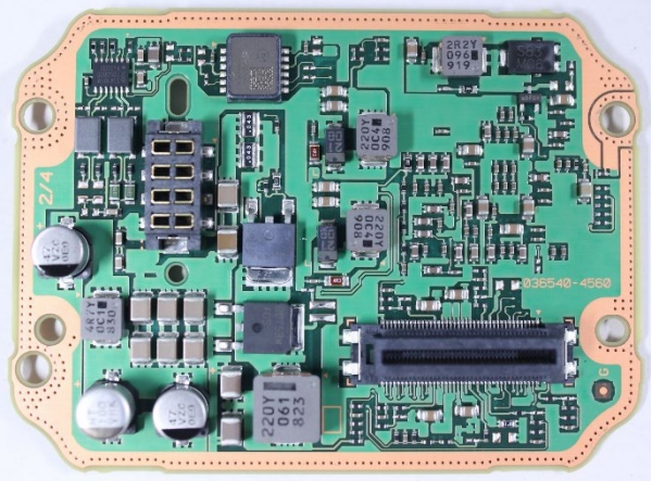
Component side A
