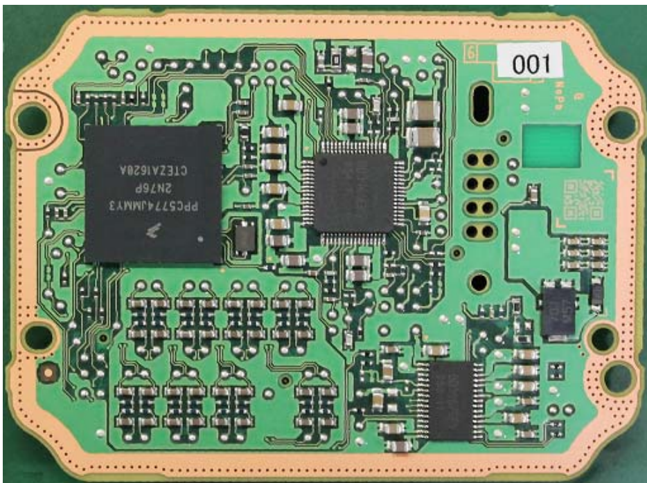
Component side B
