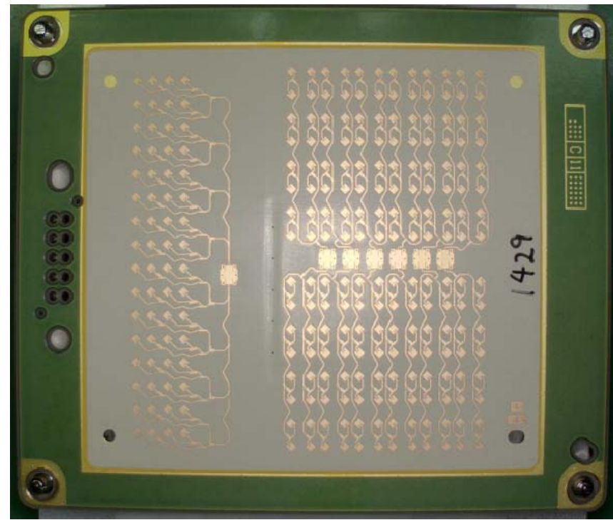
Antenna side
