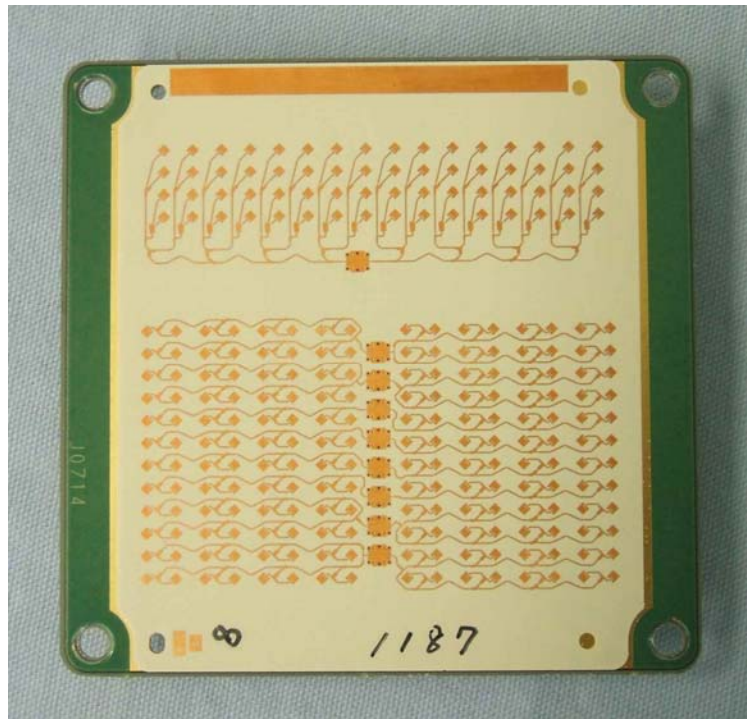
Antenna side
