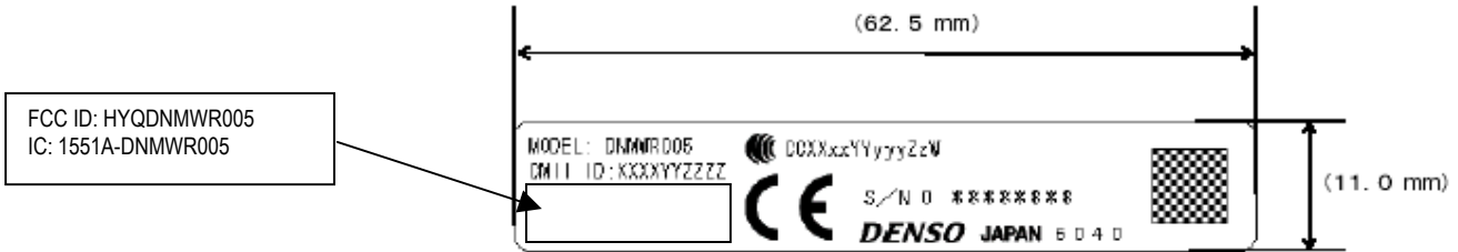
Fig. Marking Layout
