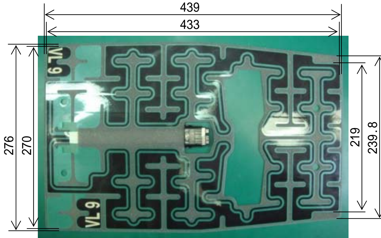
(1)Top view
