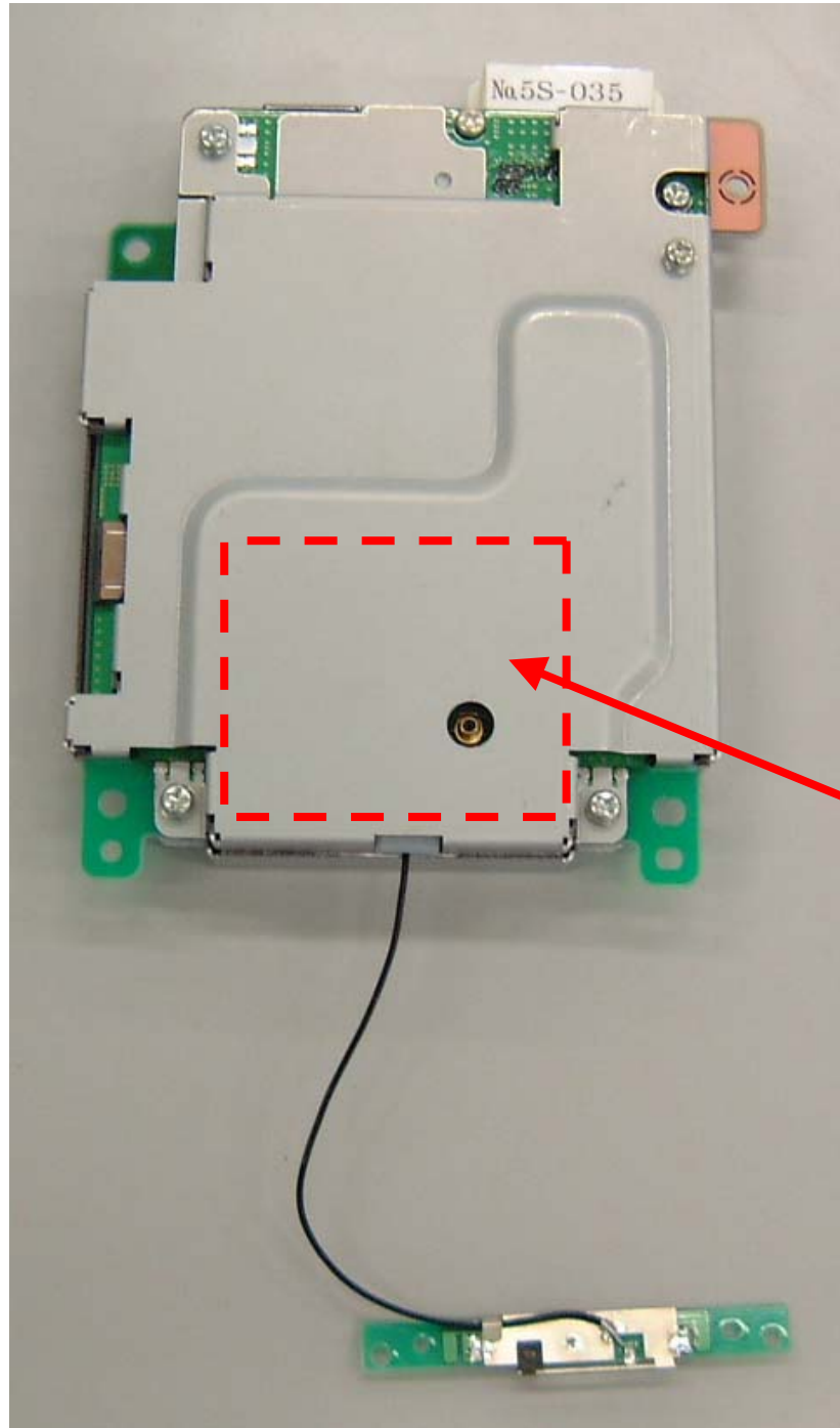
Fig. 4.5.1b. Label Location on Audio Bluetooth Hands Free Unit (BTAU02A)
