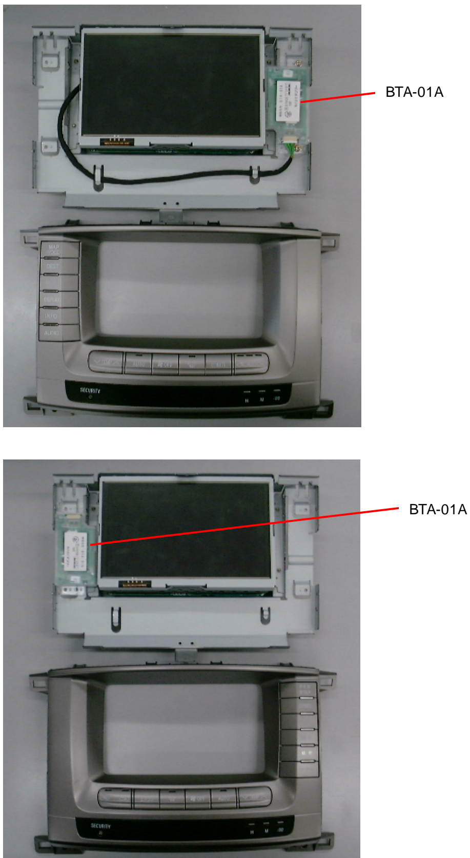
Fig. 6.3. Installation Description
