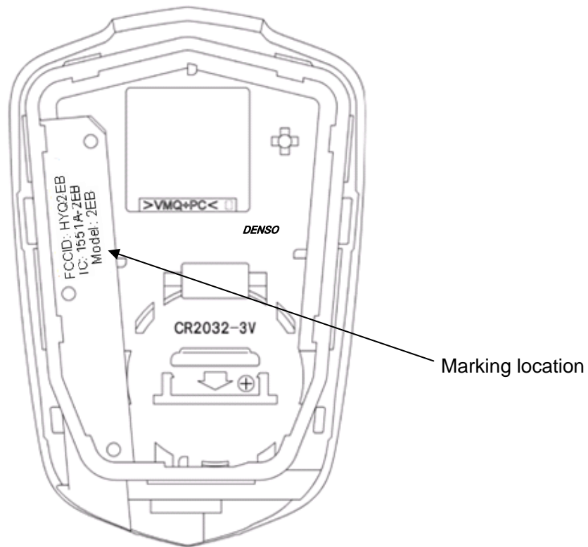
Fig: Marking location and layout
