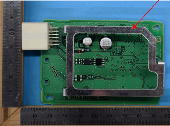
Component side with antenna
