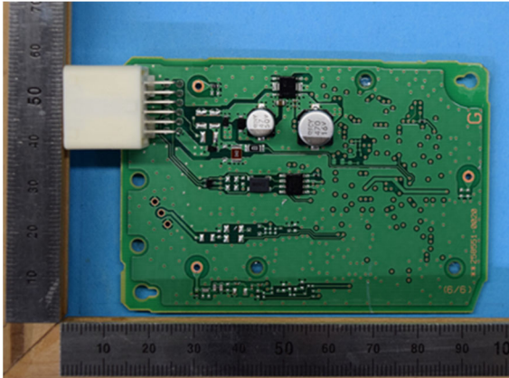
Component side without antenna
