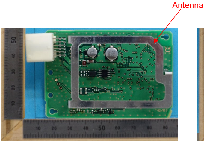
Component side with antenna
