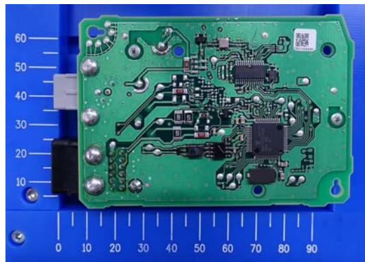
Solder side
