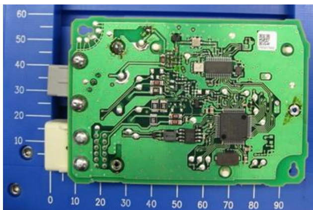
Solder Side
