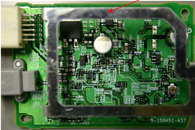
Component Side
