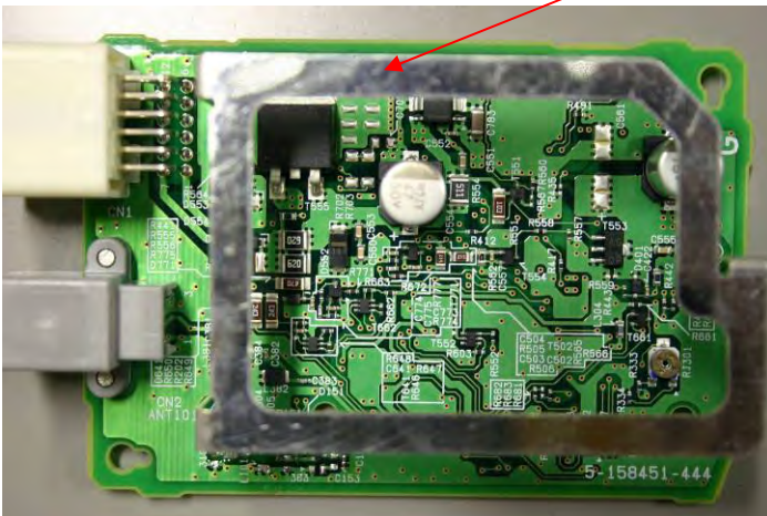
Component Side
