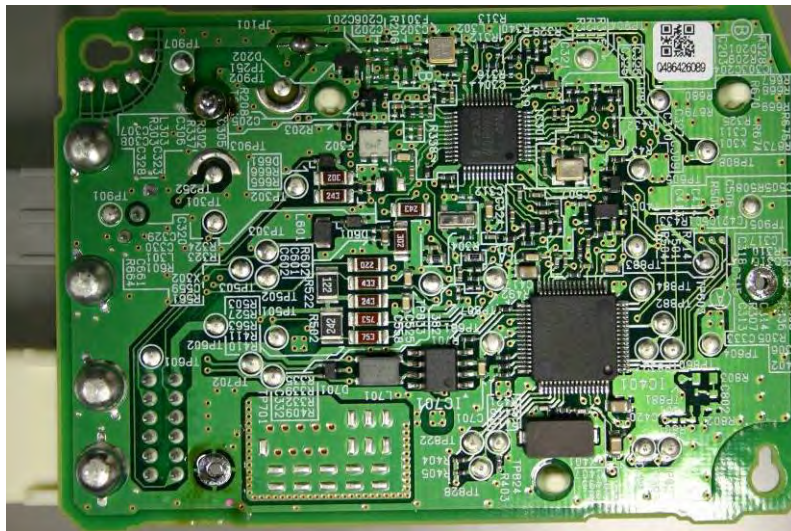
Solder Side
