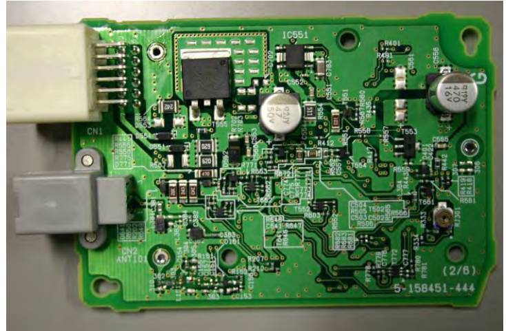
Component Side
