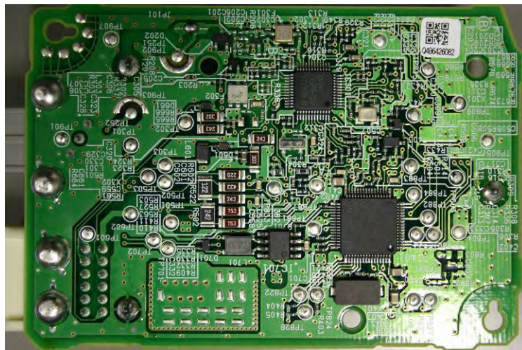
Solder Side
