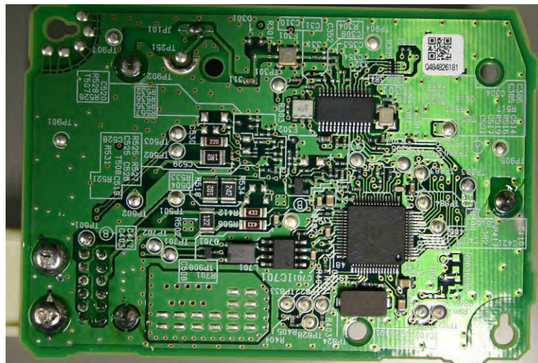
Solder Side
