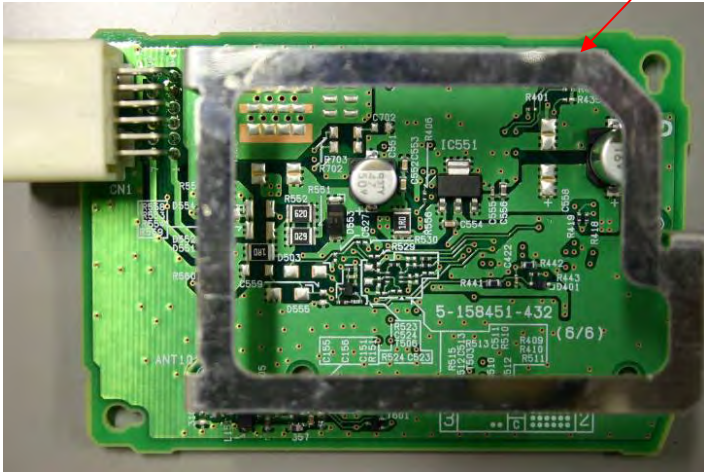
Component Side
