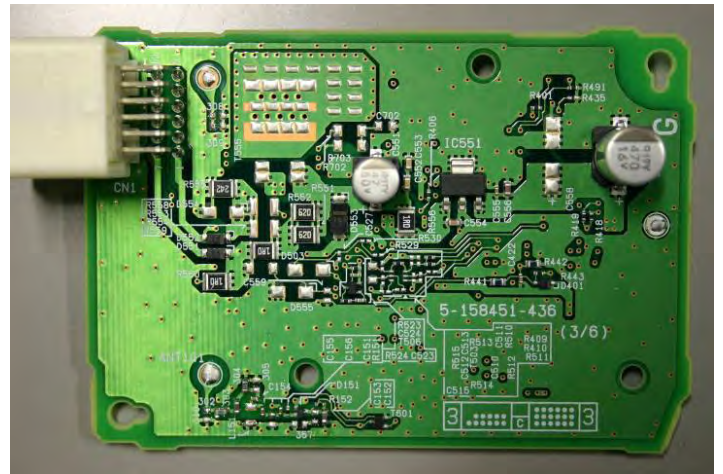
Component Side
