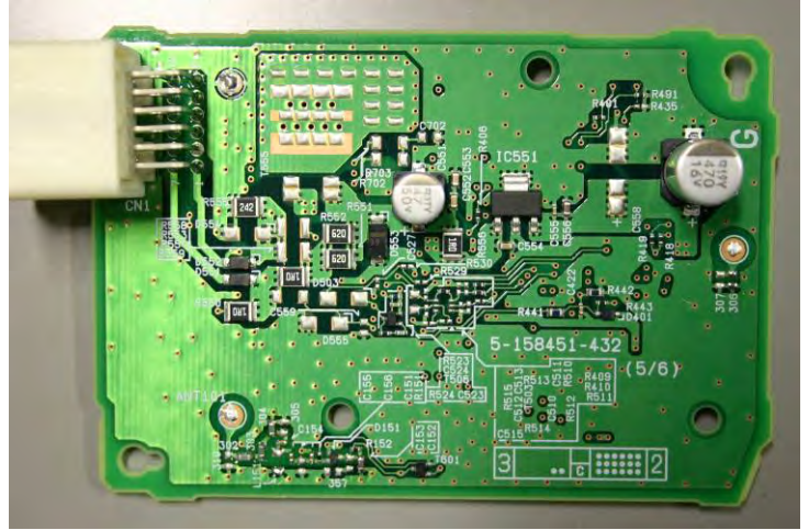
Component Side
