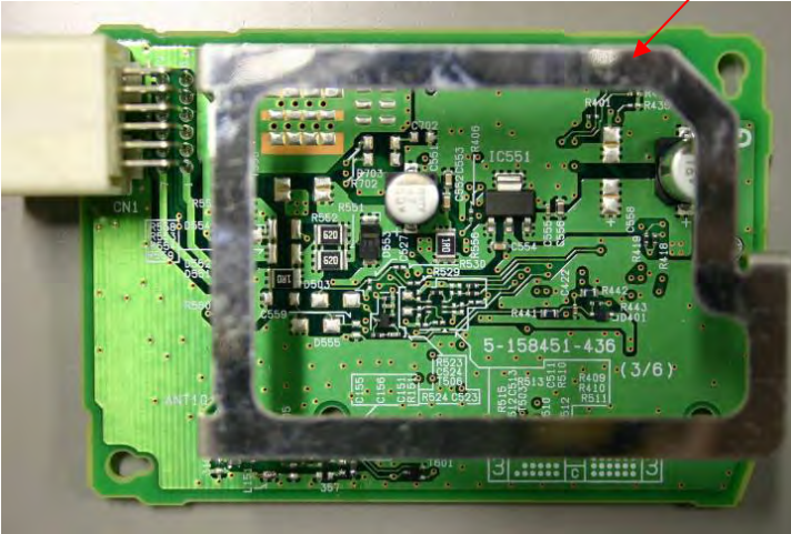
Component Side
