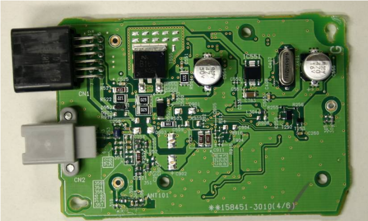
Component Side
