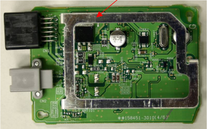
Component Side
