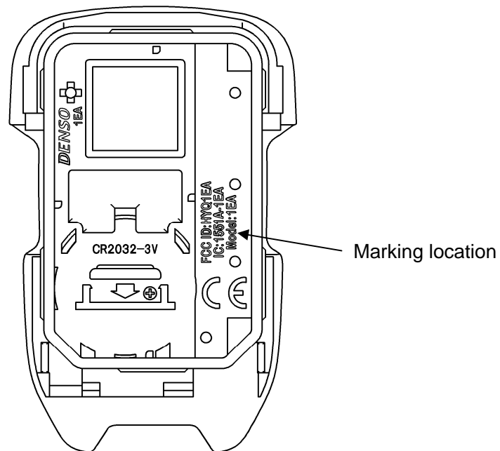
Fig: Marking location and layout
