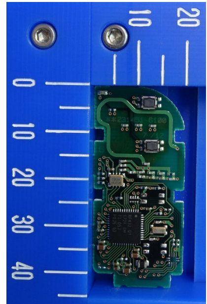
2-Button type
