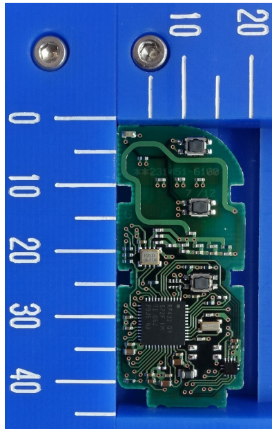
3-Button type
