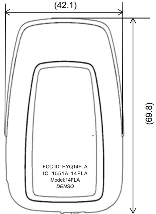
Rear View (Logo side)
