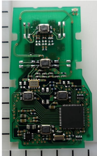
5-Button type
