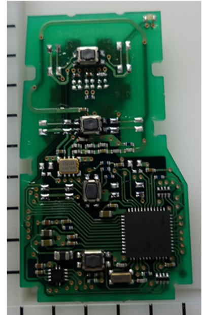
4-Button type
