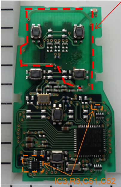
6-Button type
