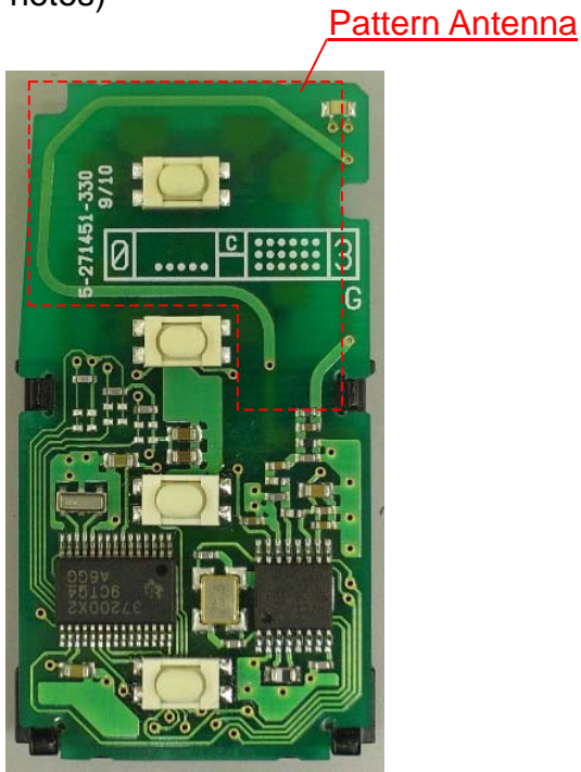
Comp. Side
