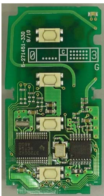
Comp. Side
