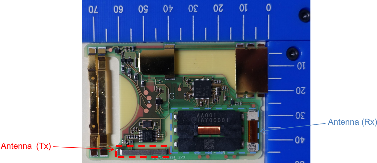
Component side
