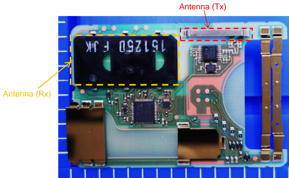
Component side
