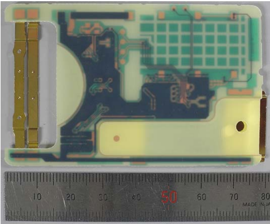
Solder Side
