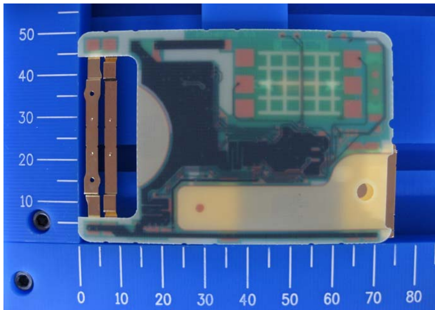
Solder side
