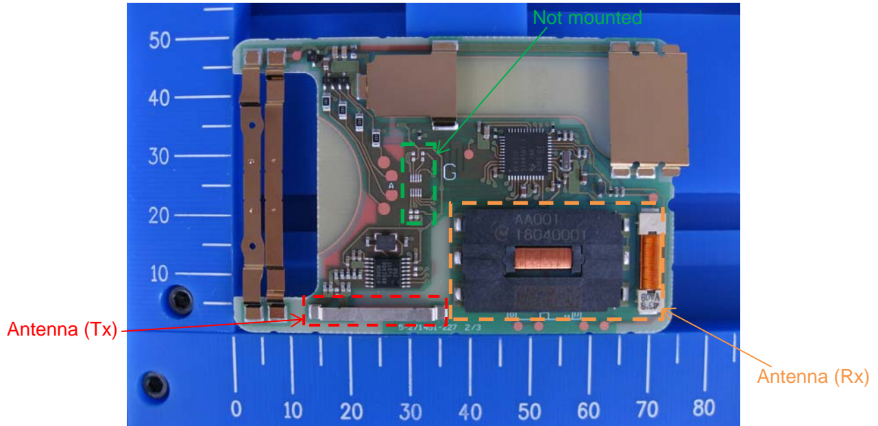
Component side
