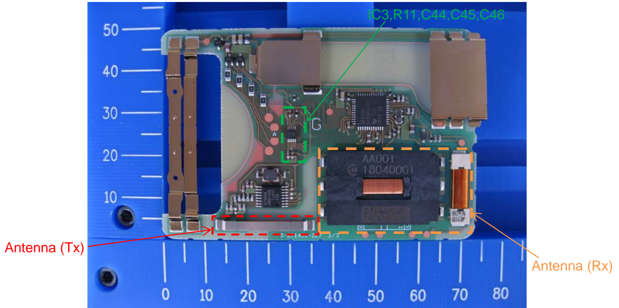
Component side
