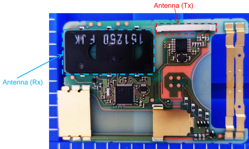
Component side
