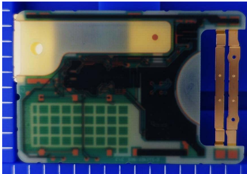
Solder side
