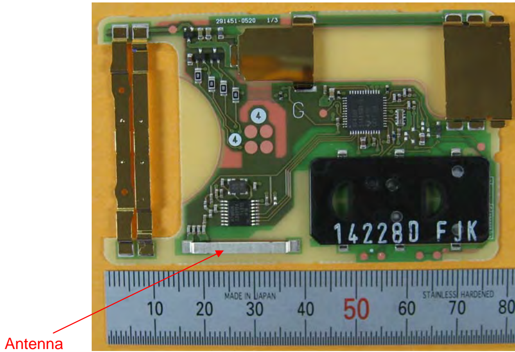
Component Side
