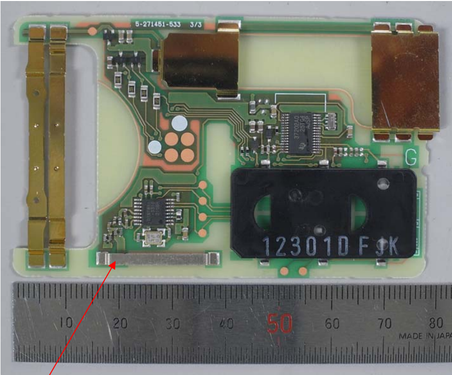
Antenna location
