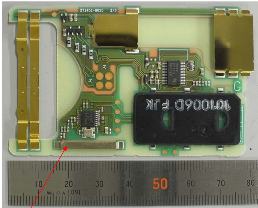
Component Side
