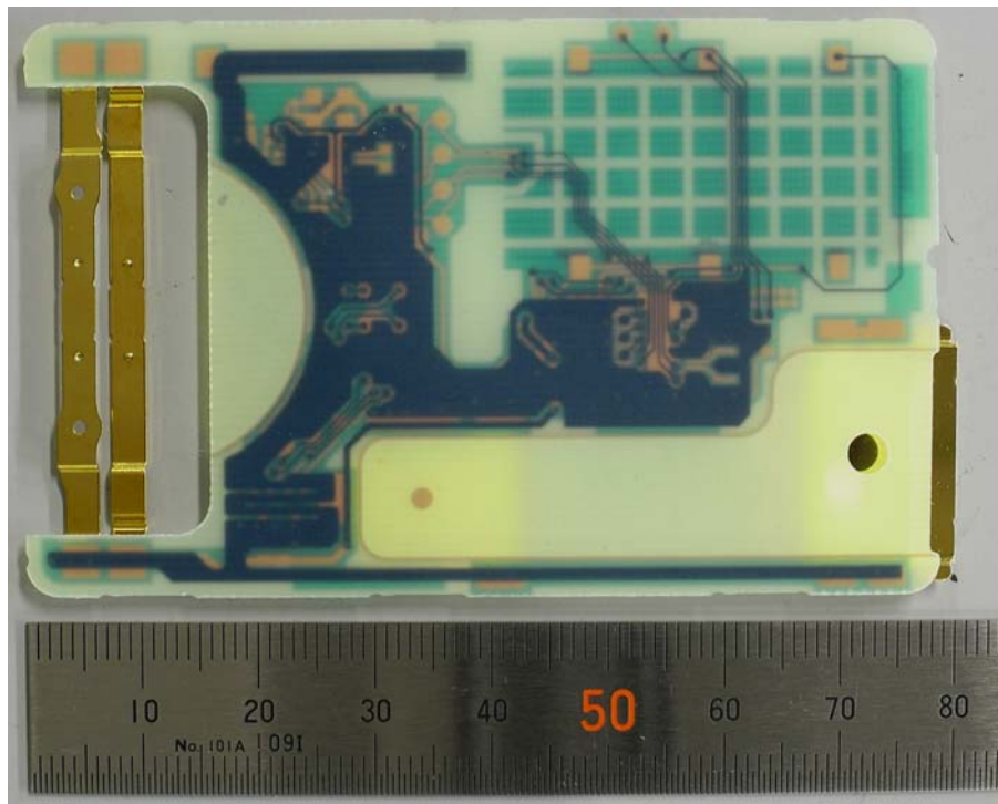
Solder Side
