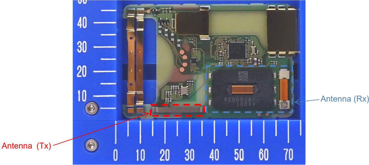
Component side
