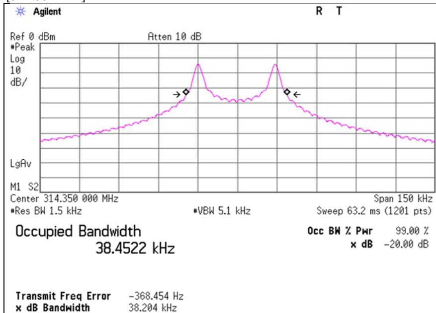
[314.35 MHz]
