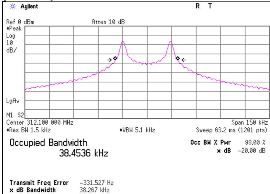
[312.10 MHz]
