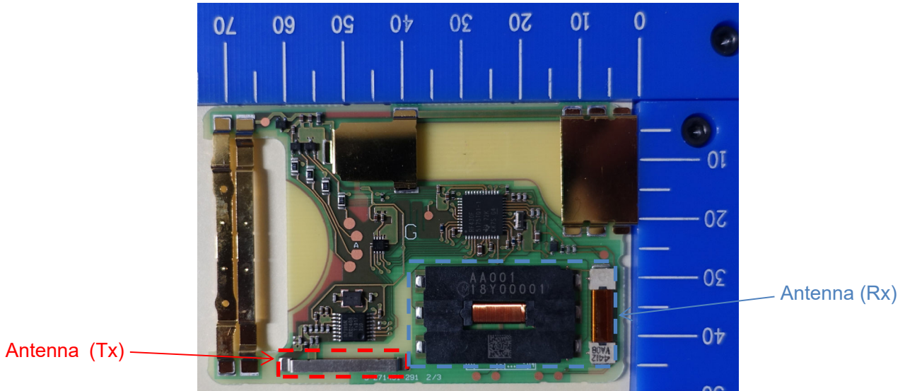
Component side
