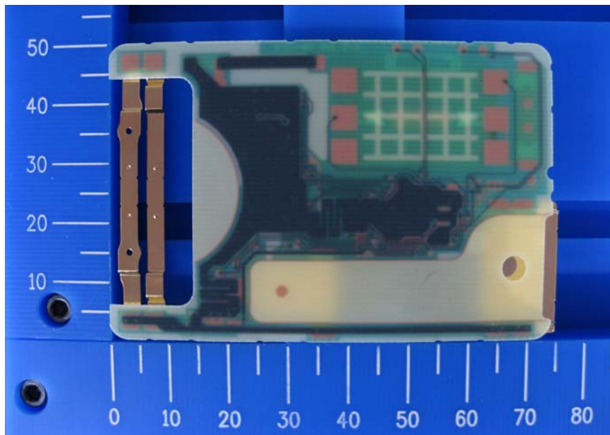
Solder side
