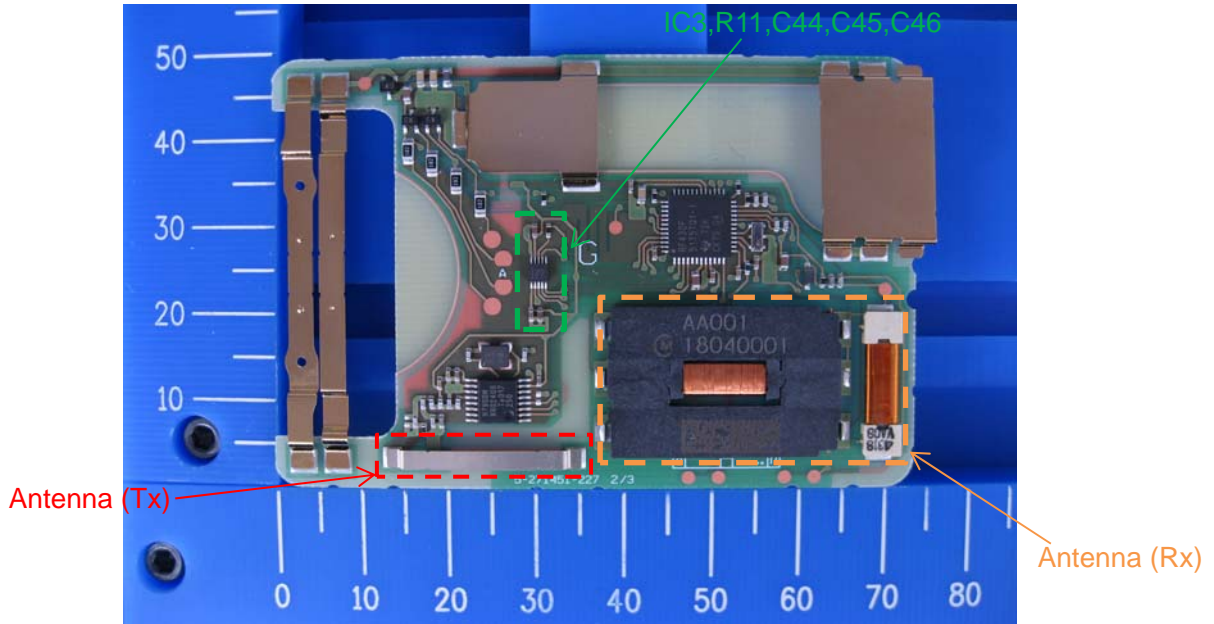
Component side
