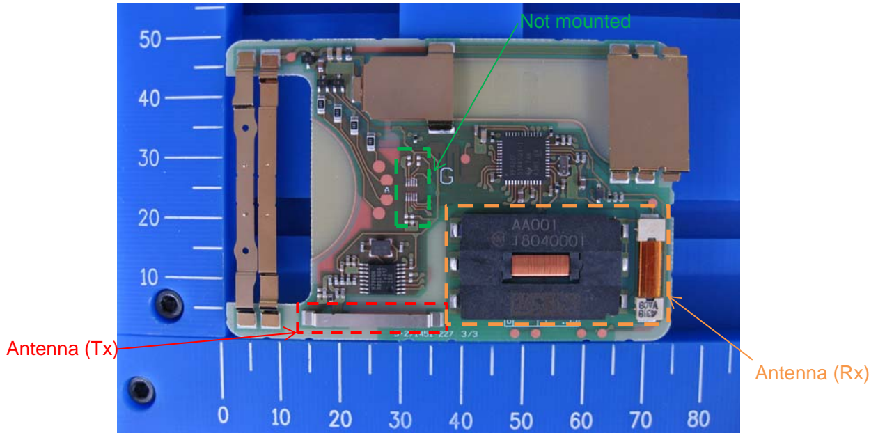
Component side
